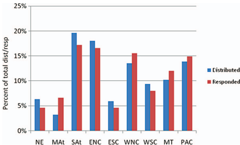
FIGURE 1. Comparison of survey distribution and response patterns. Note: NE, New England; MAT, Middle Atlantic; SAT, South Atlantic; ENC, East North Central; ESC, East South Central; WNC, West North Central; WSC, West South Central; MT, Mountain; PAC, Pacific.
