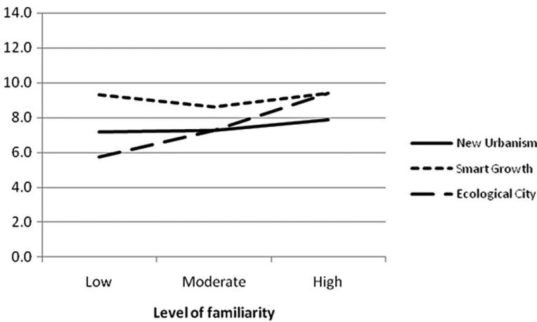
FIGURE 6. Average selection frequency by level of familiarity with the approaches (maximum of 14.0).
